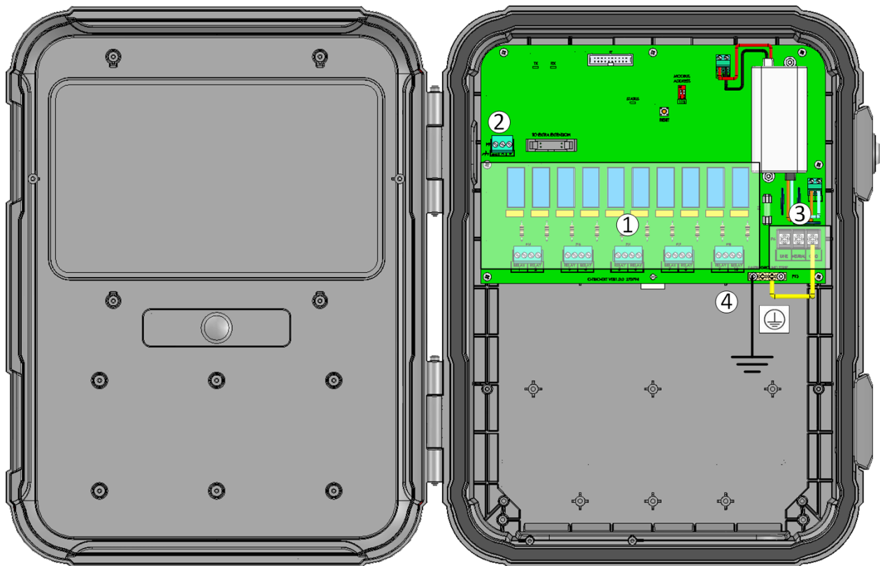
Figura 30: Board layout
