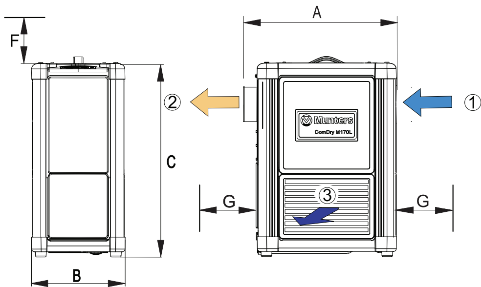
Figure 10.1 Dimensions, ComDry M170L
