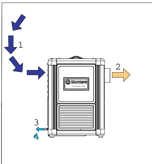
Figure 4.1 Closed system
