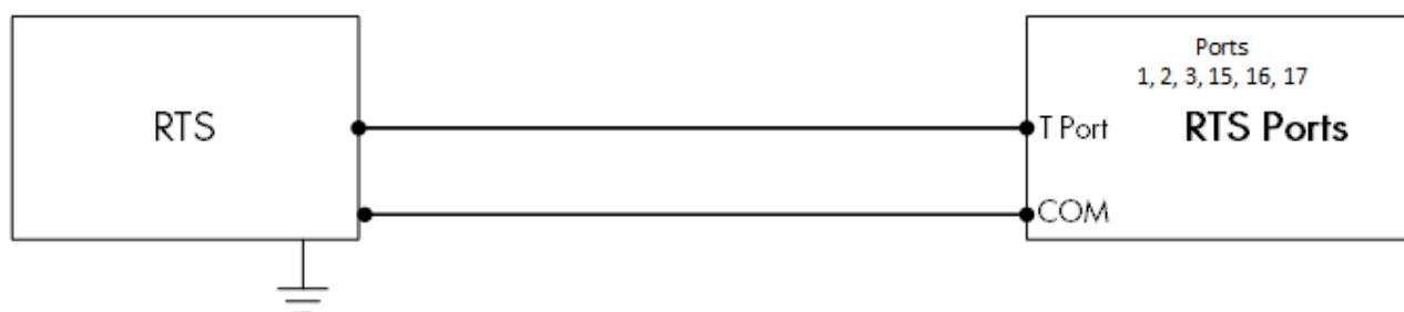
Figur 24: RTS – koblingsdiagram
