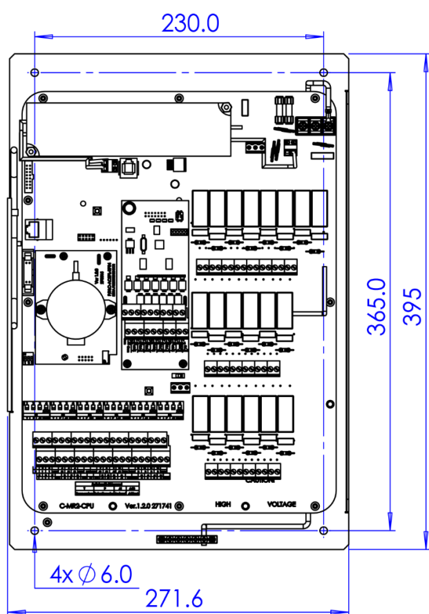
Figur 72: Bagpanel – dimensioner
