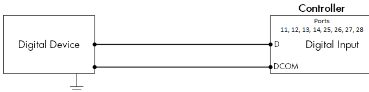
Figur 19: Koblingsdiagram for digital enhed
