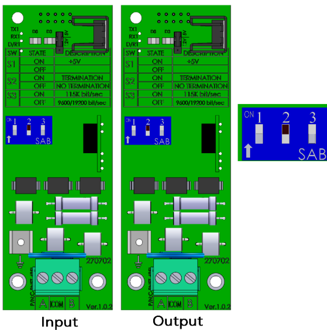
Figure 25: Repeater Termination
