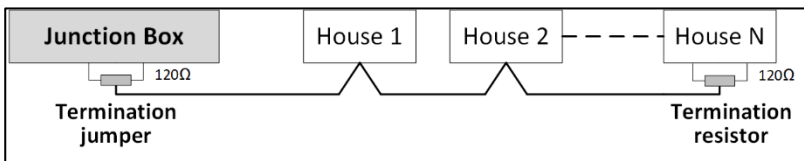
Figure 19: Topology 1: CommBox Plus/House Termination
