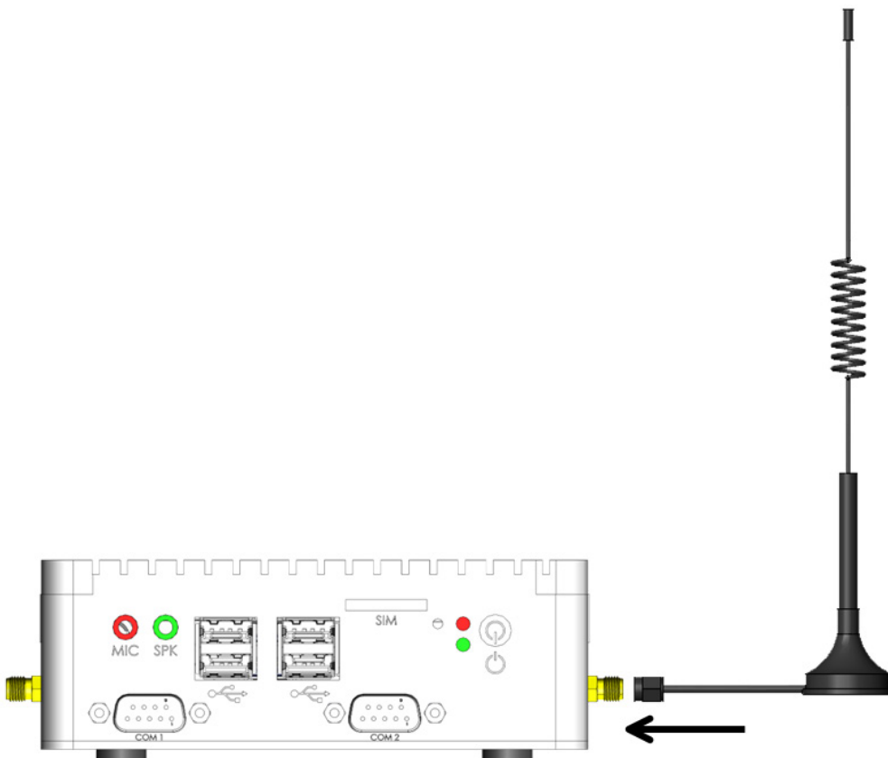
Figure 8: Antenna Connection
