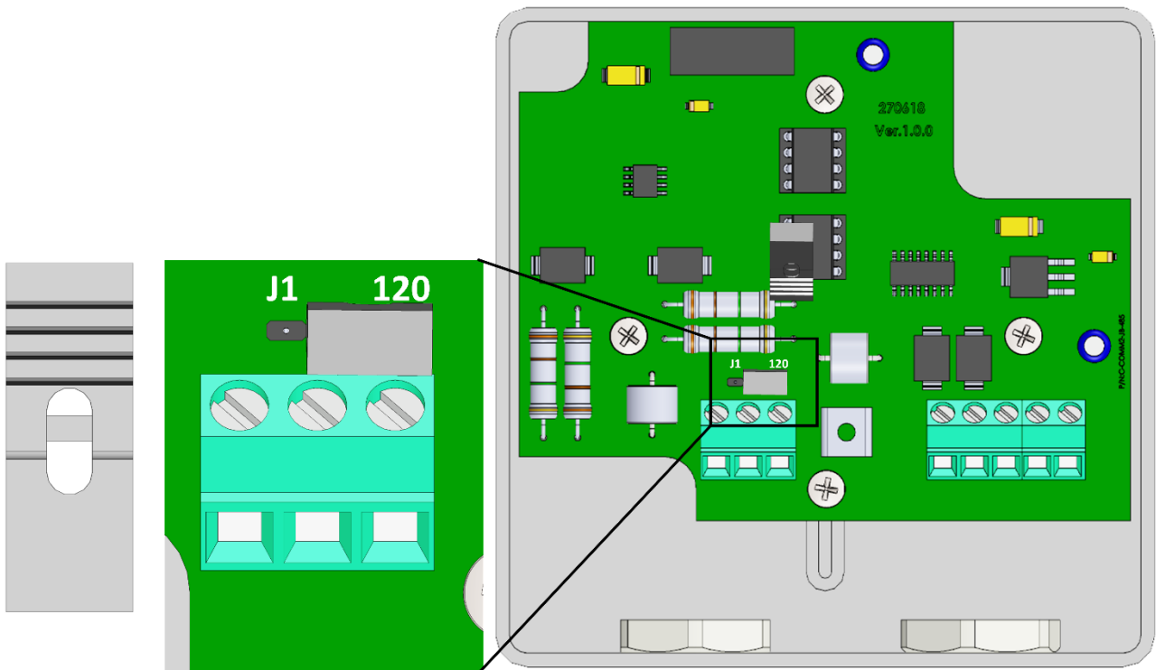
Figure 24: Junction Termination
