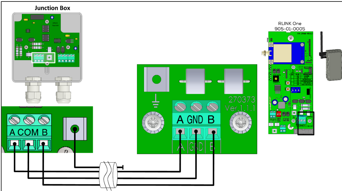
Figure 13: RLink One Wiring
