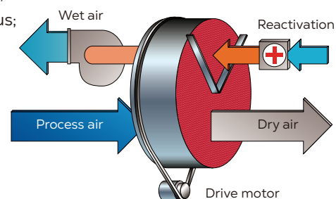
Working principle of rotor dehumidification
