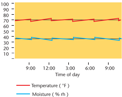
FIGURE 7.3 Simple on-off humidistats and thermostats are appropriate when the product can tolerate a range of conditions, and where the equipment is well matched to the loads.
