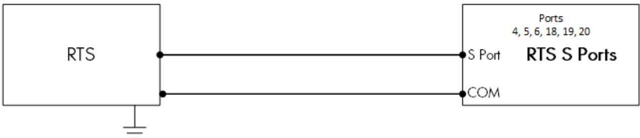
Figure 1: RTS S Port 接线图
