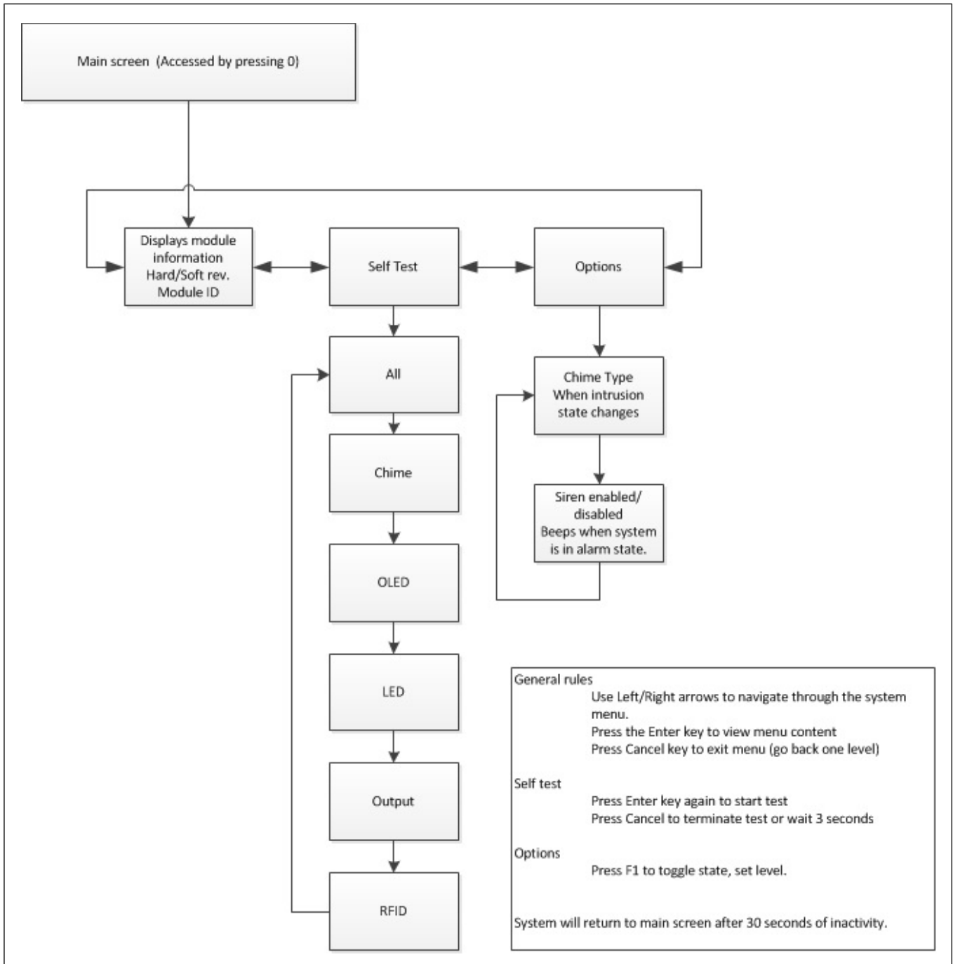
Figure A-3 Navigation in system menus
