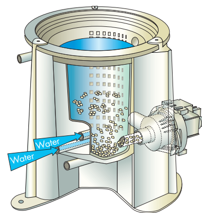
Integrated rinsing and lime collection system
