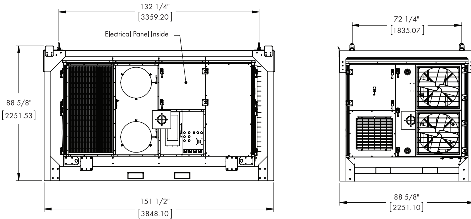
Drawing above represents DryCool 6000 model. Configuration and design is similar for other models within this product series.
